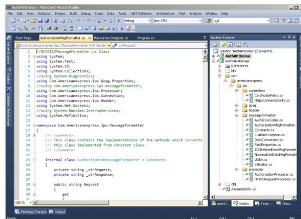
Developer Environment
